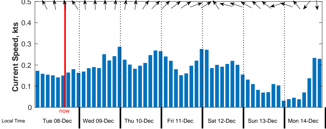
Current Forecast for TABS Buoy F from 08-Dec-2020 00:00:00 to 15-Dec-2020 00:00:00
